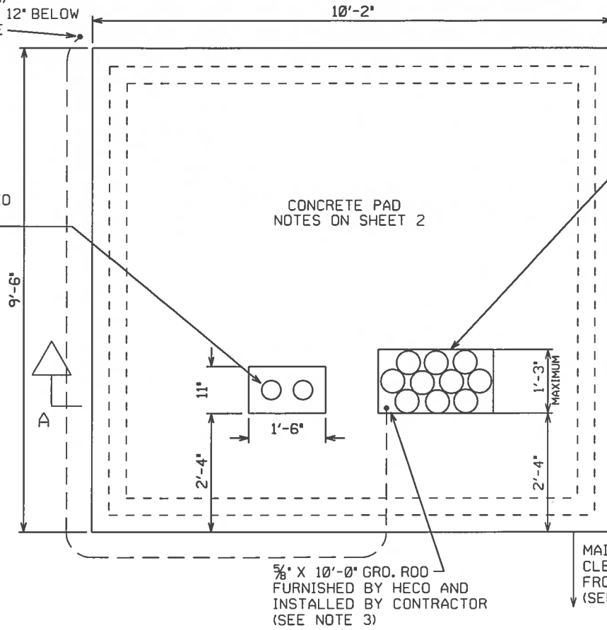
PLAN VIEW SEE NOTES ON SHEET 2
