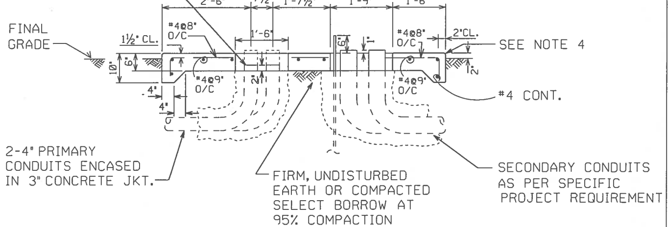
SECTION "A-A"
